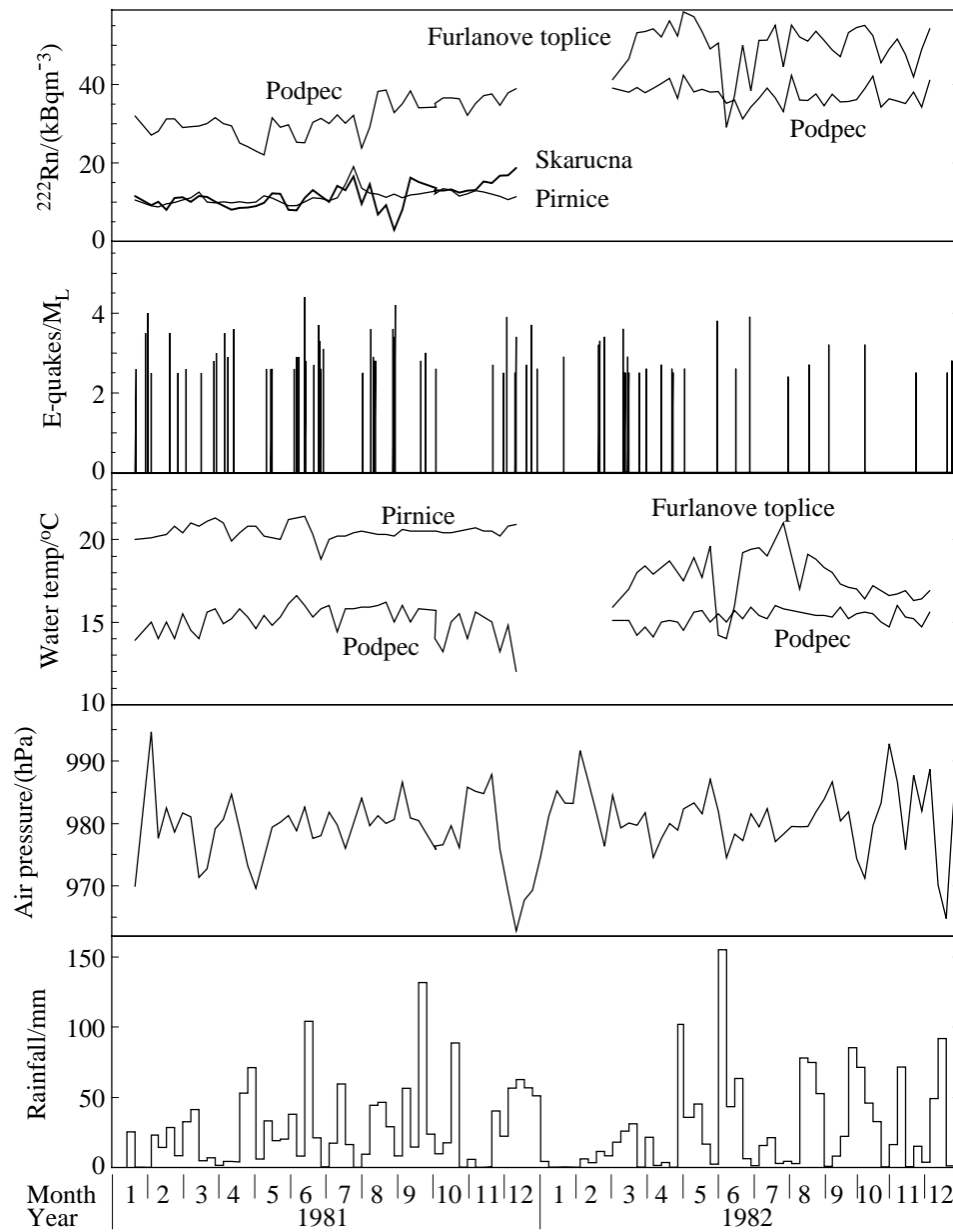
Fig. 2. Radon concentrations in selected spring waters together with seismic activity (earthquakes with epicentre distances up to 150 km), water temperature, barometric pressure, and rainfall.
